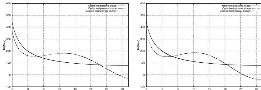
Fig. 4. Optimization of the central energies shape, penalty functions 1 (left) and 2 (right) (example)
