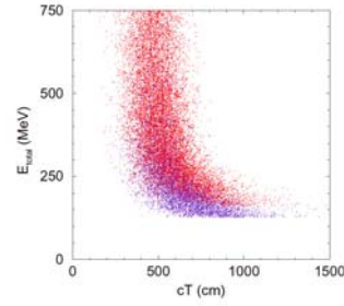
Fig. 2. Distribution of particles energies 12m from the target calculated by MARS
