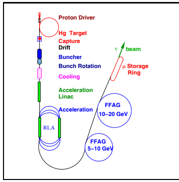
Fig. 1. Neutrino Factory Schematics (Study 2a)
