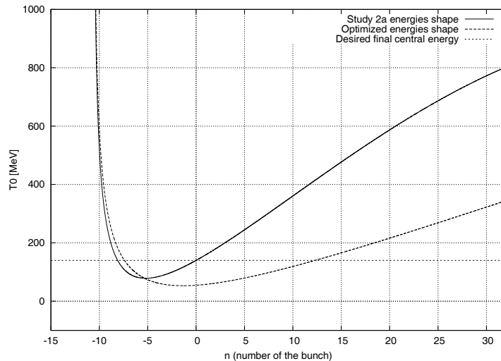
Fig. 5. Optimization of the central energies shape, penalty function 2 (Study 2a parameters)
