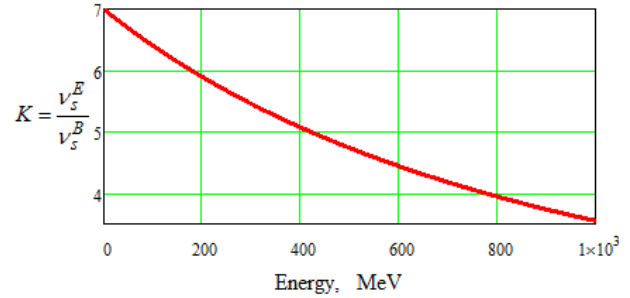
Figure 1: The ratio \nu_s^E / \nu_s^B vs beam energy.
