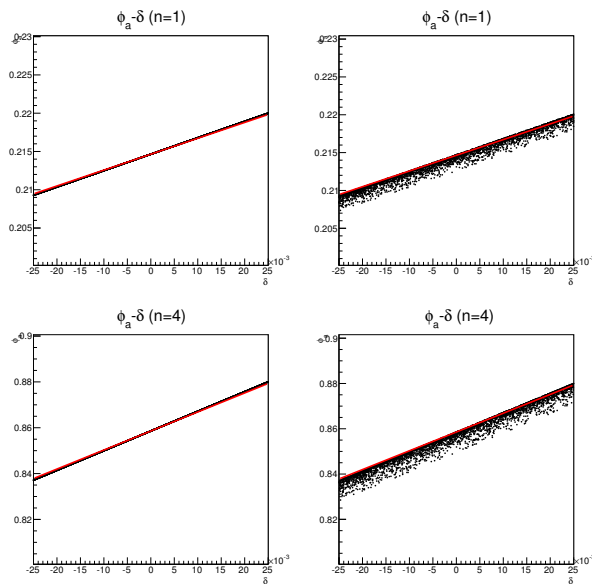
Figure 6: Spin precession angle versus momentum offset for muons travelling inside a homogeneous ring.
