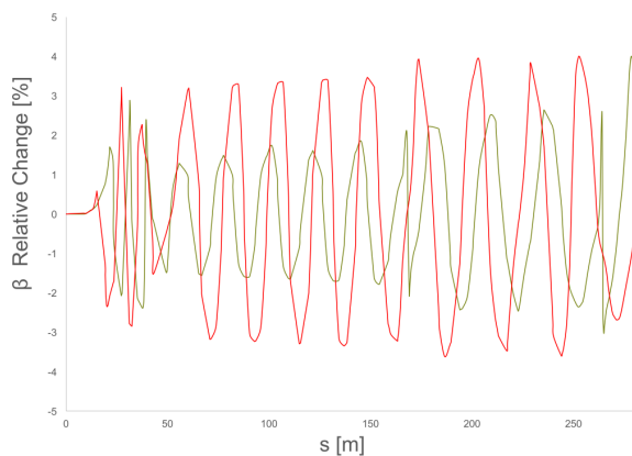
Figure 3: Fringe field effects on beta functions along M2/M3 beamlines. The graphs correspond to the relative difference between calculated x (green) and y (red) beta functions with and without fringe fields.
