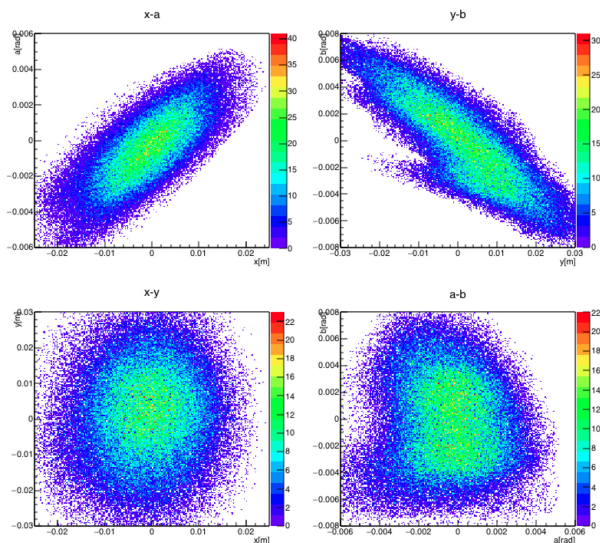
Figure 5: Beam distributions at the end of M2/M3 beamlines.
