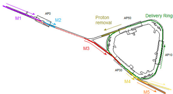
Figure 1: Muon campus beamlines at Fermilab.
