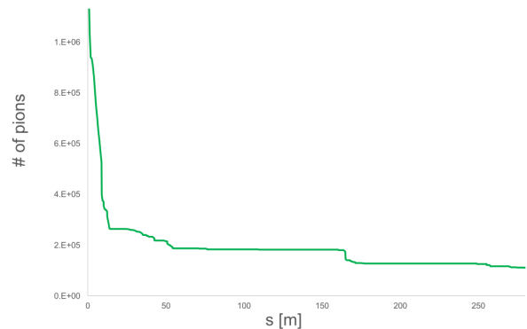
Figure 4: Pions transmission in M2/M3 beamlines. Our results are in good agreement with G4BL and BMAD simulations performed by D. Stratakis, M. Korostelev et al. (the Muon g - 2 Collaboration).
