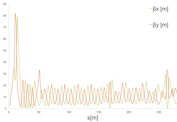
Figure 2: M2M3 beta functions.
