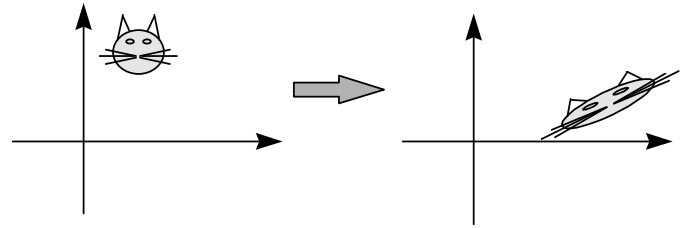
Liouville's Theorem
