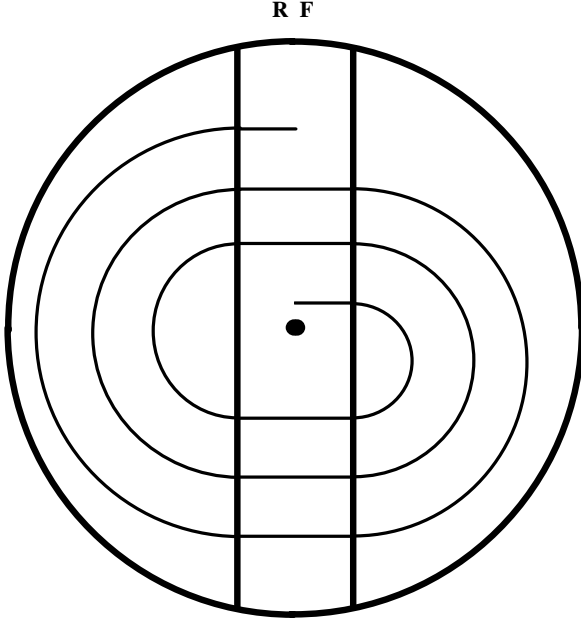
The Cyclotron
