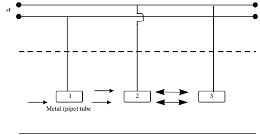
The Linac
