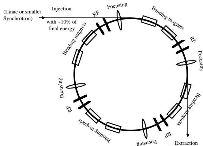
The Synchrotron
