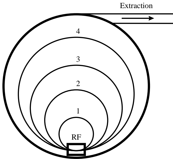
The Microtron
